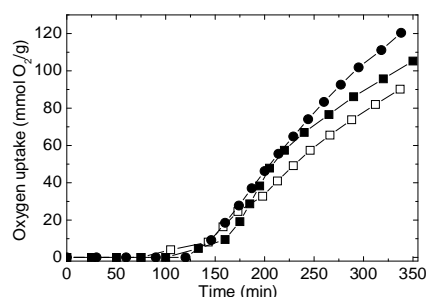
Figure 1. The dependencies of oxygen uptake on degradation time for unirradiated samples consisting of i-PP and CaCO 3 nanoparticles coated with stearic acid. ( \square ) control; ( \blacksquare ) 5 % loading; ( \bullet ) 25 % loading.
